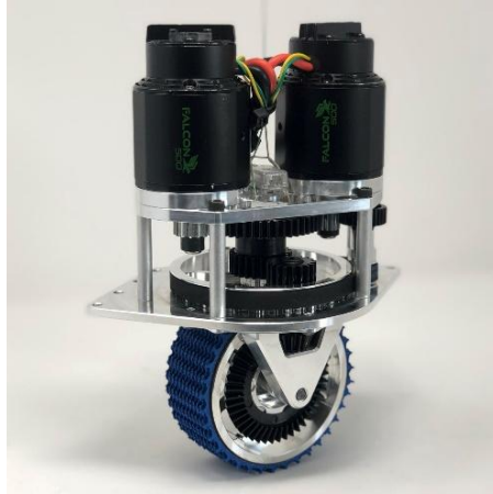
Gambar 4. Modul Swerve Drive
